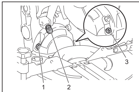
► 1. Right 45° bevel angle adjusting bolt 2. Pointer 3. Left 45° bevel angle adjusting bolt
